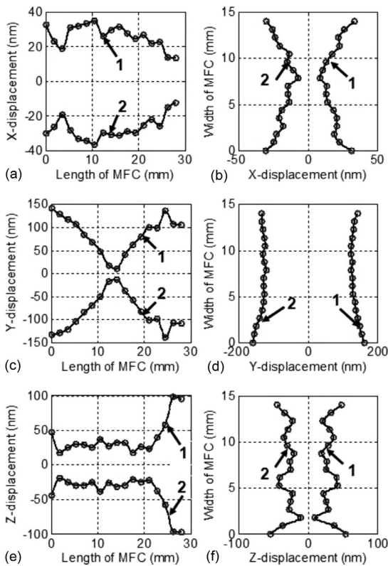
Figure 5: Positive and negative 3D (X, Y and Z) displacements along the length and width, measured at edges of MFC-P1: a) X displacements along the length and b) along the width, c) Y displacements along the length and d) along the width, e) Z displacements along the length and f) along the width (1- measured positive displacements, 2- measured negative displacements)
