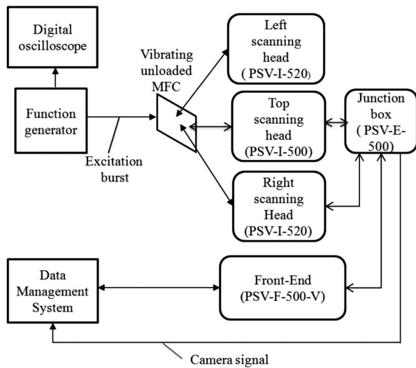
Figure 3: Experimental set-up for 3D displacement measurement using Polytec PSV-500-3D-HV laser vibrometer
