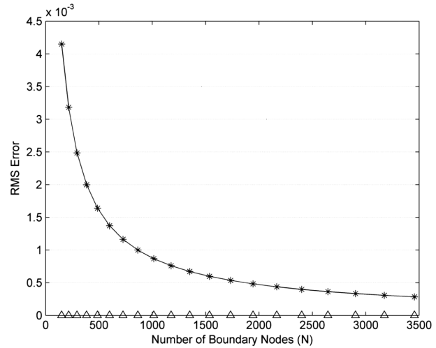
Figure 5: The relationship between the RMS errors and the number of boundary nodes for the deformation case, calculated by NMFS. R=d/3 (+: e_x , x: e_y , Δ: e_z ).
