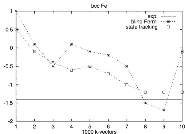
Figure 1: The calculated MAE for bcc Fe with respect to the number of k-vectors in units of \mu\text{eV}/\text{atom} . The horizontal line represents the experimental data
