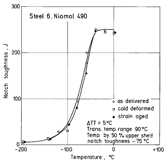
Figure 11: Steel 3. Influence of testing temperature on notch toughness
