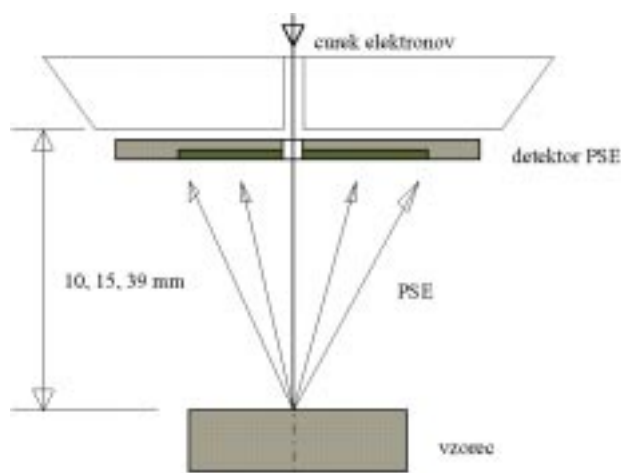
Slika 3: Shema meritve relativnega koeficienta PSE Figure 3: Backscattered coefficient measurement arrangement
